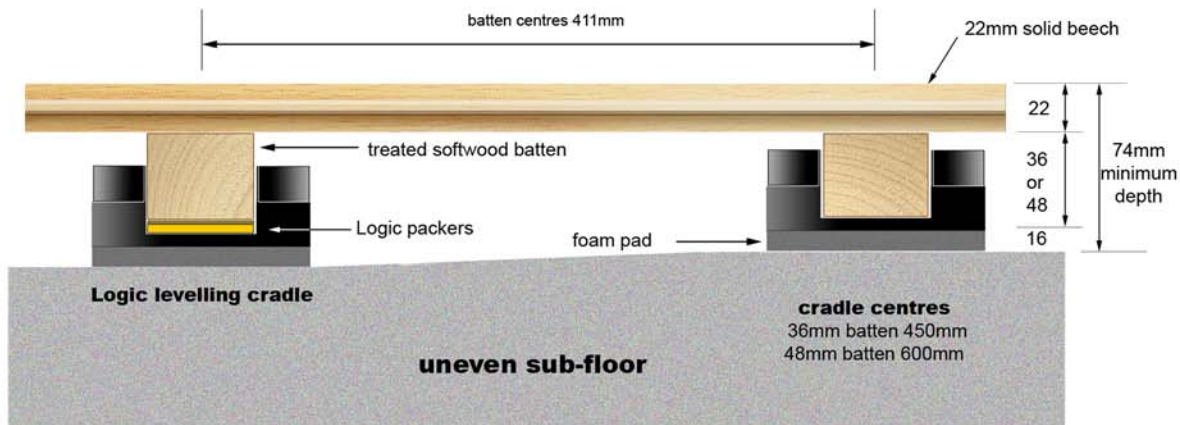
cradle system for use where sub-floor is not level or extra depth is required
