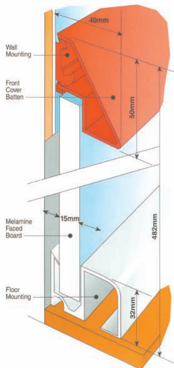
Sounding Board ("Tin") System
